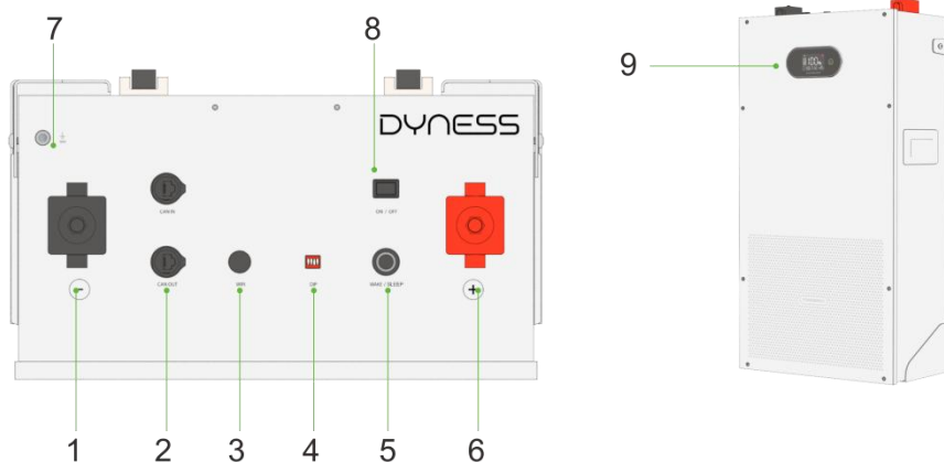
Figure 2-1 PowerBrick SC the Sketch of Front Interface
