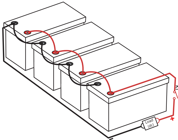
Figure 5-2 Parallel Application: 1S4P,25.6V 400Ah
