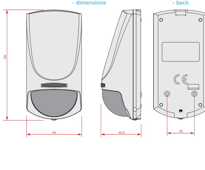
XIRP200H, XDTP200H, XDTP200HM, XTTP200H - dimensions
