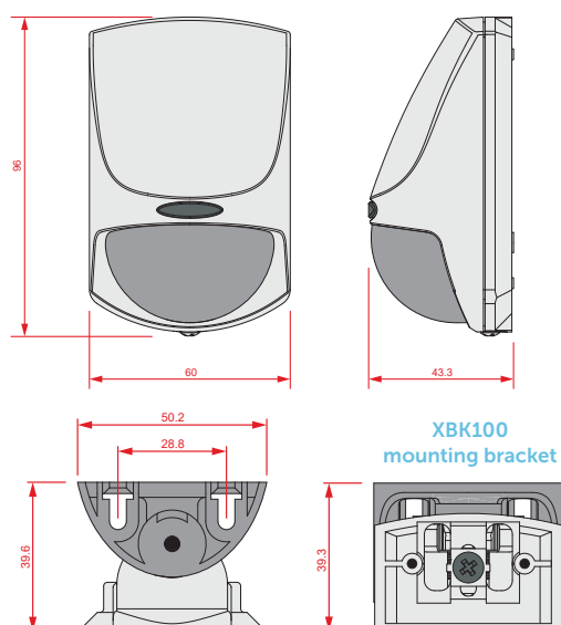
XIRP100H, - dimensions
