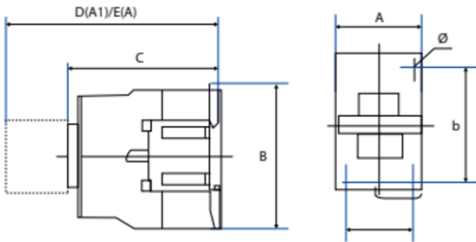
LC1-D09 AL 32
