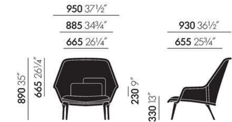
Slow Chair Knit
