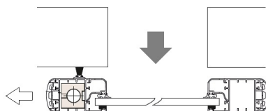
Simple break-out system for active panel without door stop
