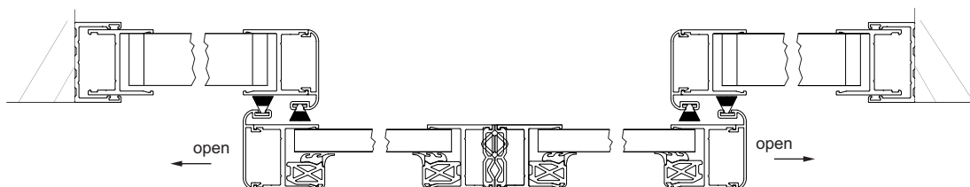
Double active + fixed panels
