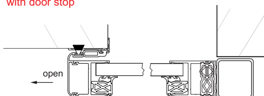
Single active panel with door stop
