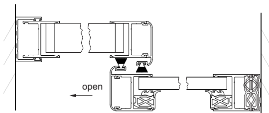
Single active + fixed panels with door stop
