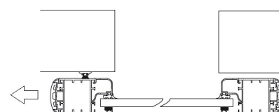
Active panel without door stop and without break-out system
