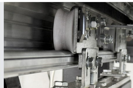
Carriages KIT
