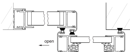
Double active panels
