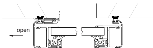
Single active panel without door stop
